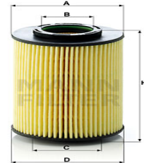
Oil Filter HU 822/5 x EM-10153
